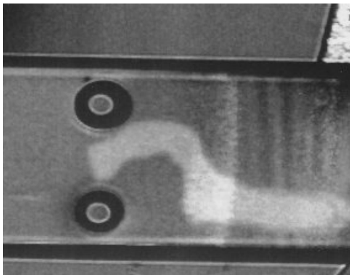
Fig. b: Interface between Chrome and metal, a delamination is visible Frequency: 25 MHz, Image width: 36 mm
