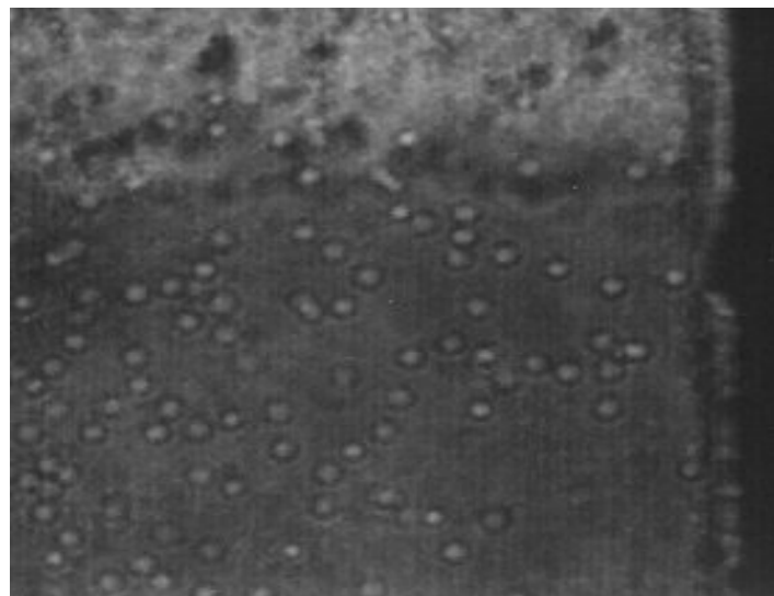
Fig. b: Lacquer above synthetic material, defects are visible Frequency: 25 MHz, Image width: 20 mm
