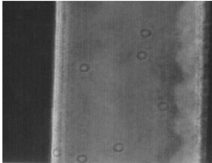
Fig. a: Lacquer above synthetic material, defects are visible Frequency: 25 MHz, Image width: 20 mm
